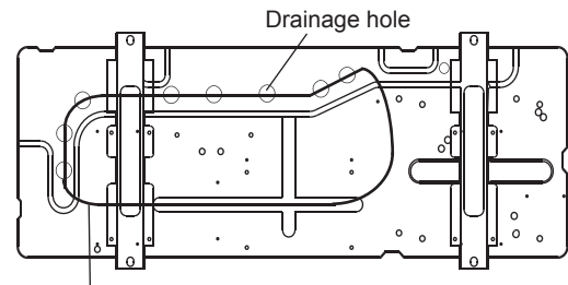
Electric heating belt of the chassis
